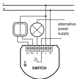
Fig.1 Wiring diagrams for Fibaro Switch.
