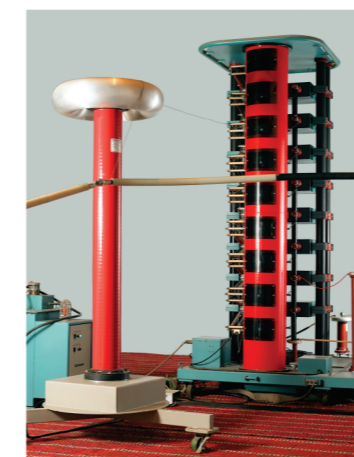
Impulse Test Set Up
